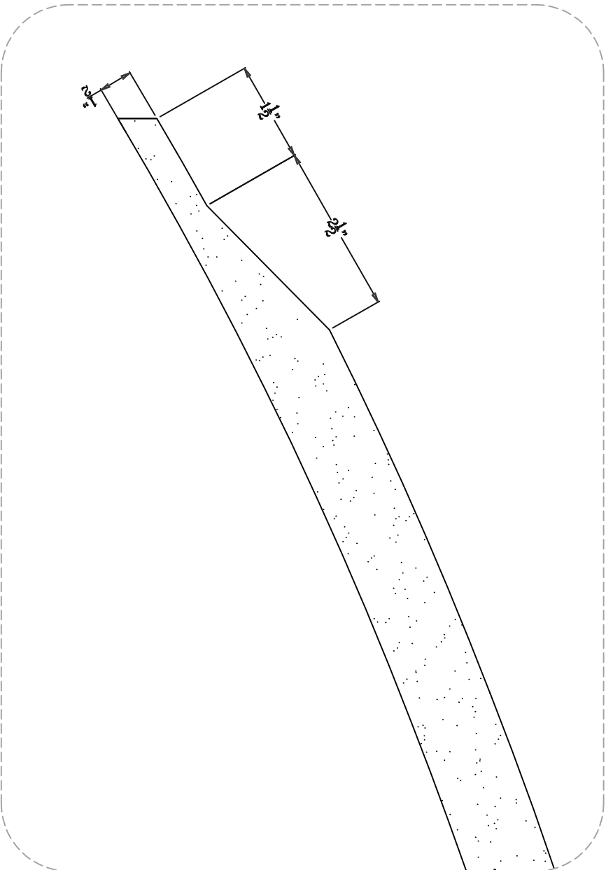
DETAIL - 5' ARCH ARCH REF. N.A. SCALE 6"=1'0"
